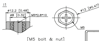
A Detail Drawing
